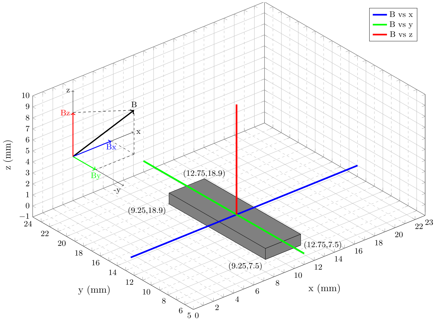
Appendix 1 : 3D analysis of bra magnet showing plotting lines of the main magnetic field strengths relative to magnet orientation (x - blue, y - green and z - red axes)
